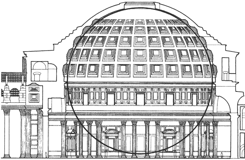
Figure 8.1 Cross-section of the Pantheon
