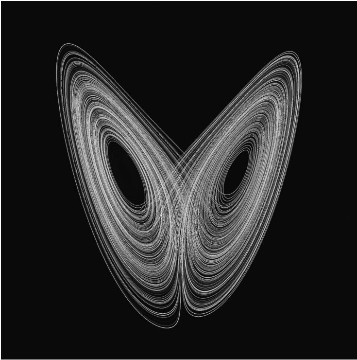
Figure 2.2 Lorenz attractor
